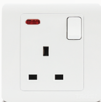
71407 13A 1 gang switched socket, SP+ neon 71411 13A 1 gang switched socket, DP+ neon
