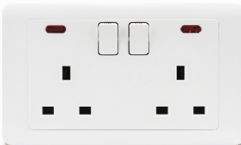
71408 13A 2 gang switched socket, SP+ neon 71412 13A 2 gang switched socket, DP+ neon
